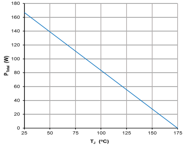
Figure 4. Power Derating
