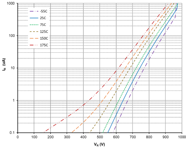
Figure 3. Reverse Characteristics
